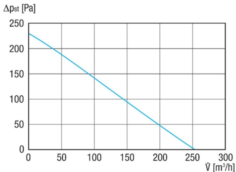
RadonTec AlphaBlower RAD 125 - Characteristic curve
